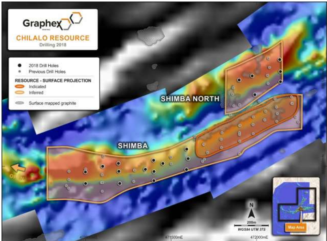
Figure 1. Location of drilling at Chilalo
